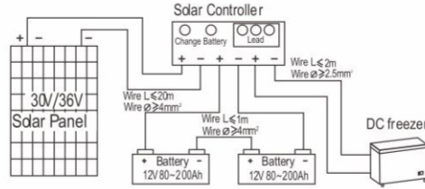
24V Solar freezer system
