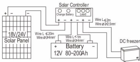
12V Solar freezer system
